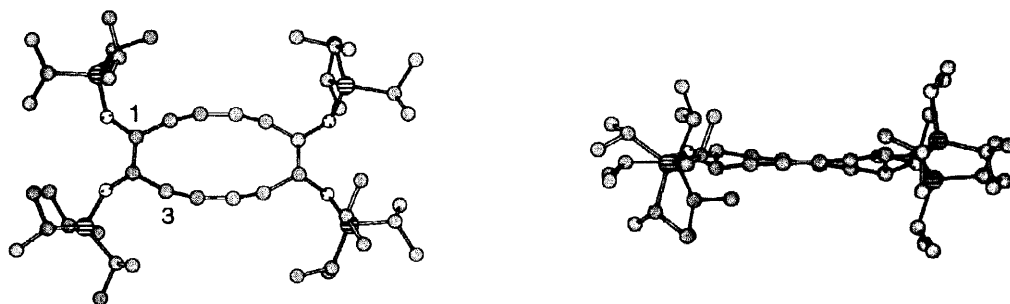
Figure 1. X-ray Crystal Structure of Tetrayne 6 . 10
